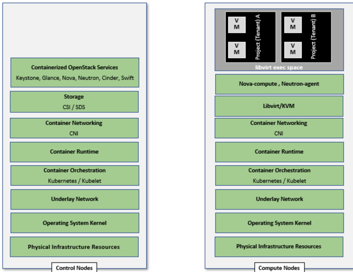
Figure 10 Containerized OpenStack Services Topology.
