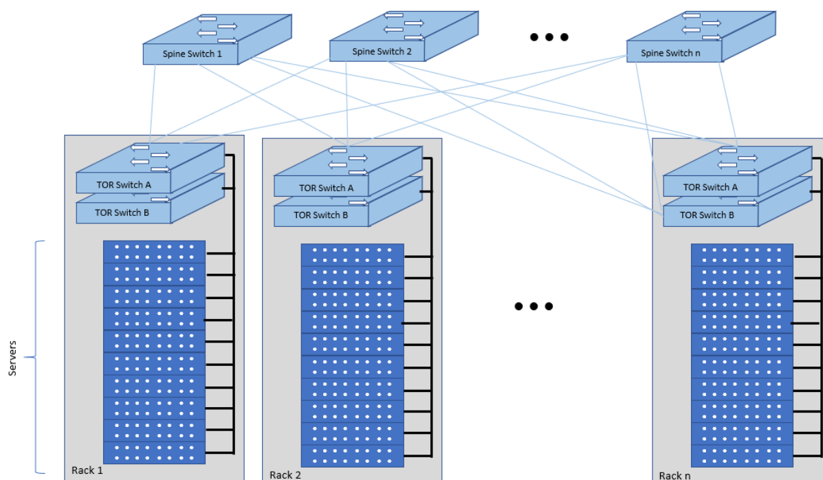
Figure 3 Network Fabric – Physical
