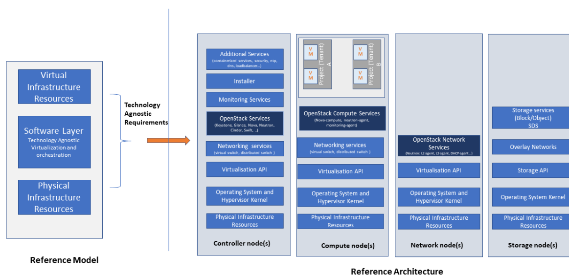
Figure 2 OpenStack Services Topology
