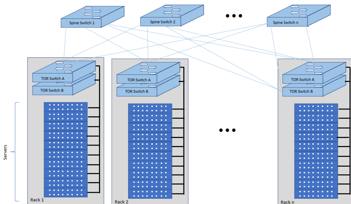
Figure 3 Network Fabric - Physical
