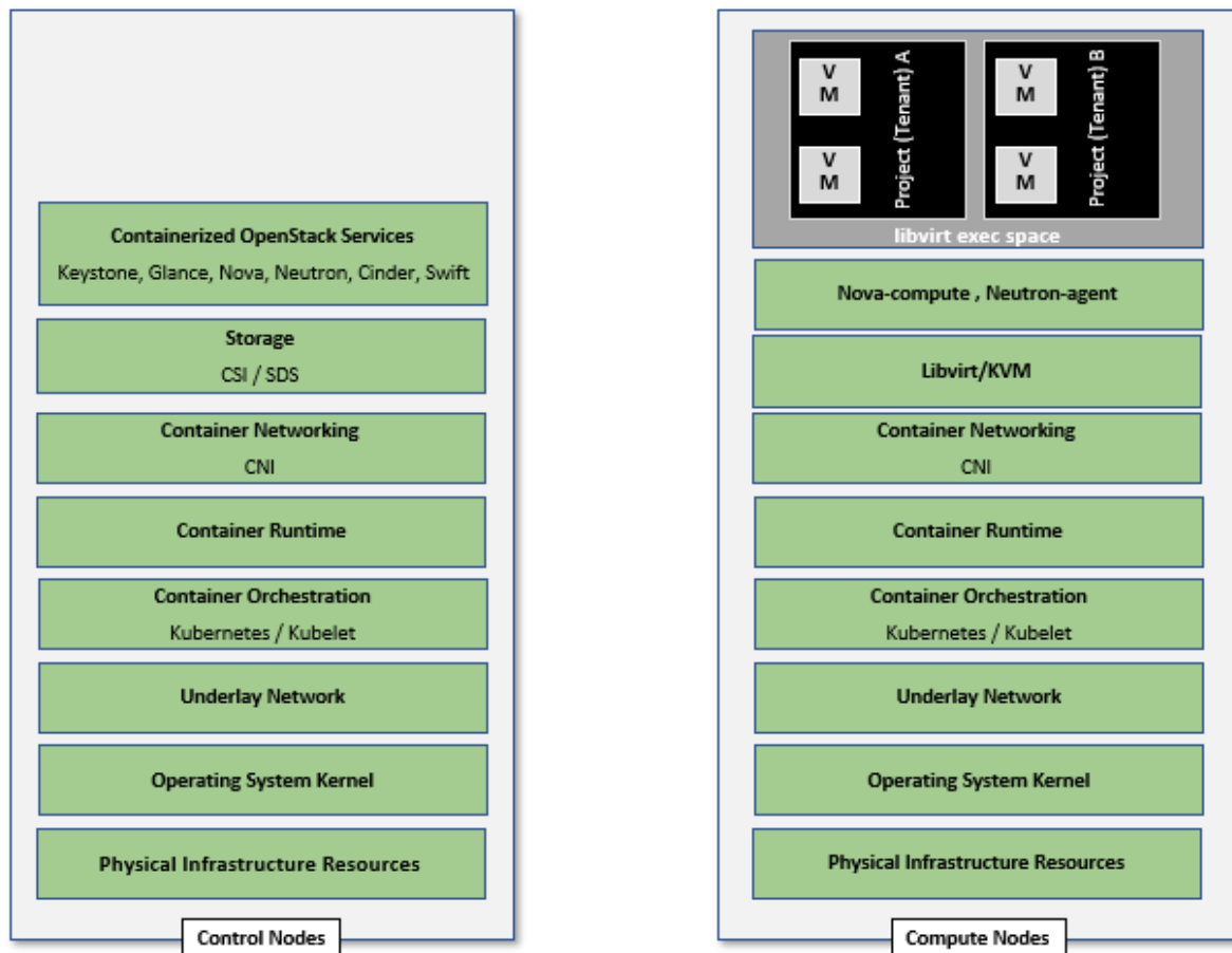
Figure 10 Containerised OpenStack Services Topology
