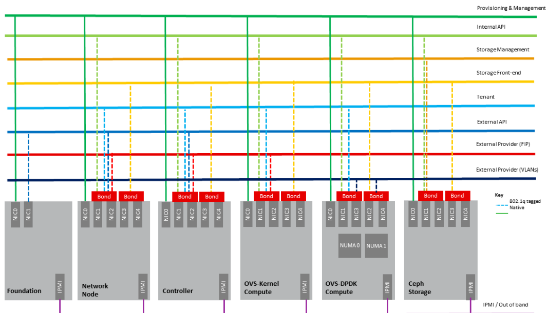
Figure 8 Indicative OpenStack Network Layout
