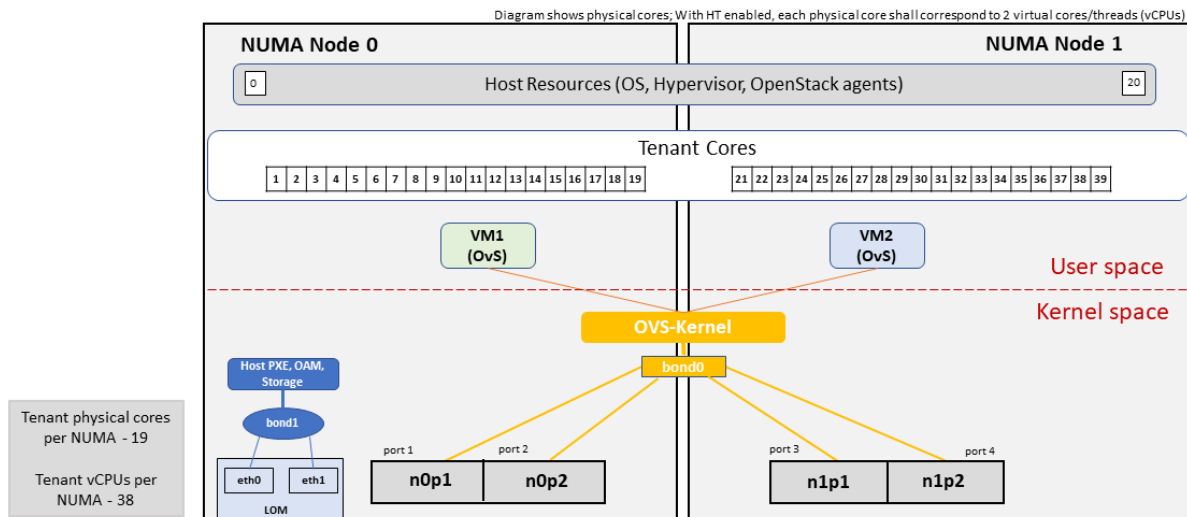
Figure 4 Basic Profile Host Configuration (example and simplified)
