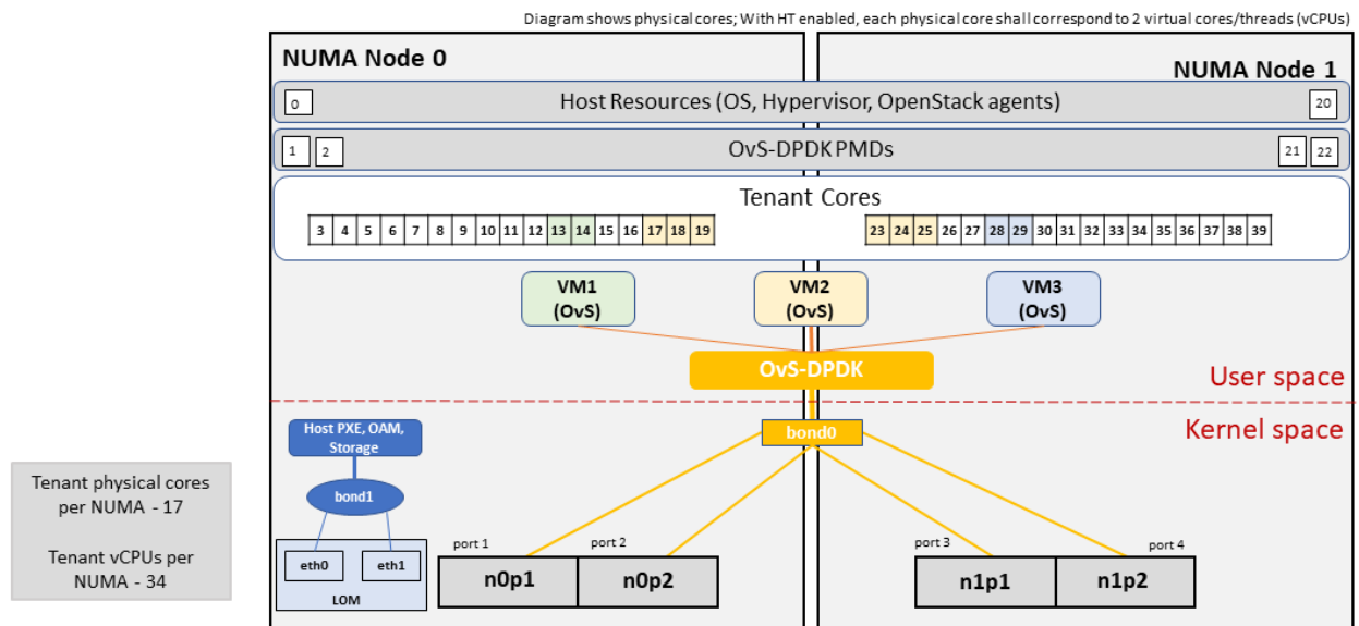
Figure 4-3: High Performance Profile Host Configuration with DPDK acceleration (example and simplified)
